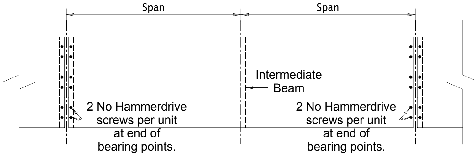
DETAIL ON FIXING TO STEEL BEAMS ~ Scale N.T.S. (HAMMERDRIVE SCREWS)
