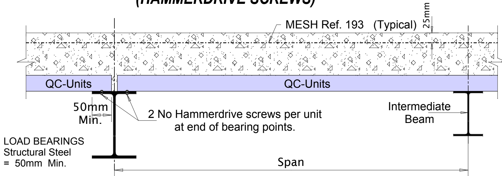
DETAIL ON FIXING TO STEEL BEAMS ~ Scale 1 : 5 (HAMMERDRIVE SCREWS)
